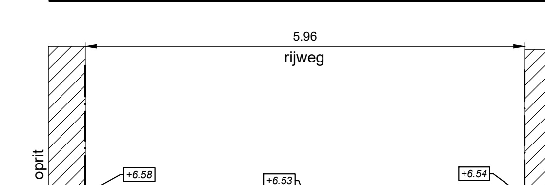
TYPE DWARSPROFIEL 8-8 school 1/50
